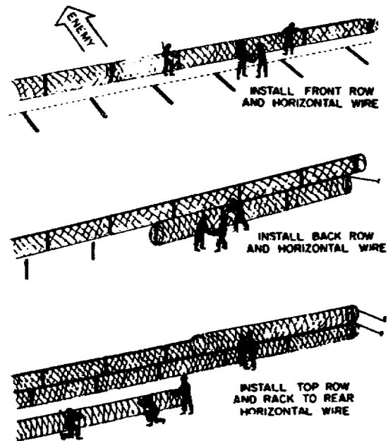
Figure 4-27. Installing concertina.
